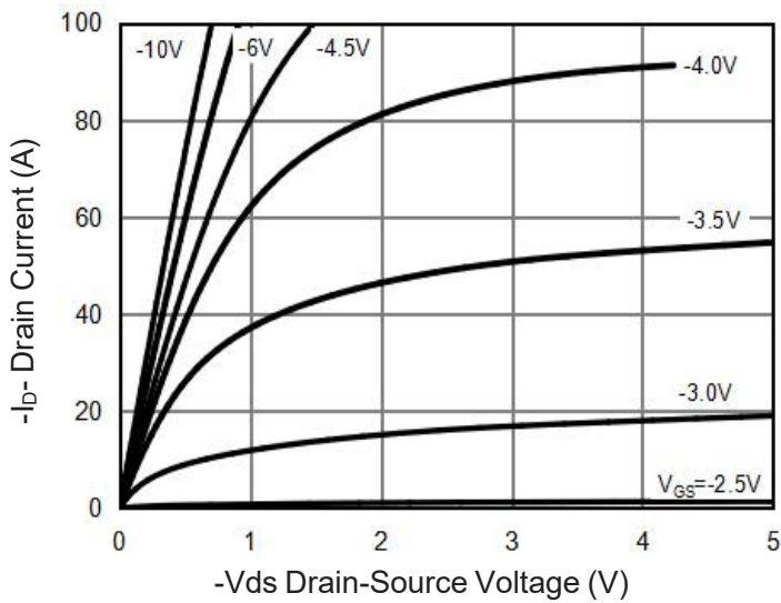
Figure 5 Output Characteristics
