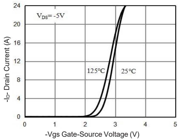
Figure 6 Transfer Characteristics
