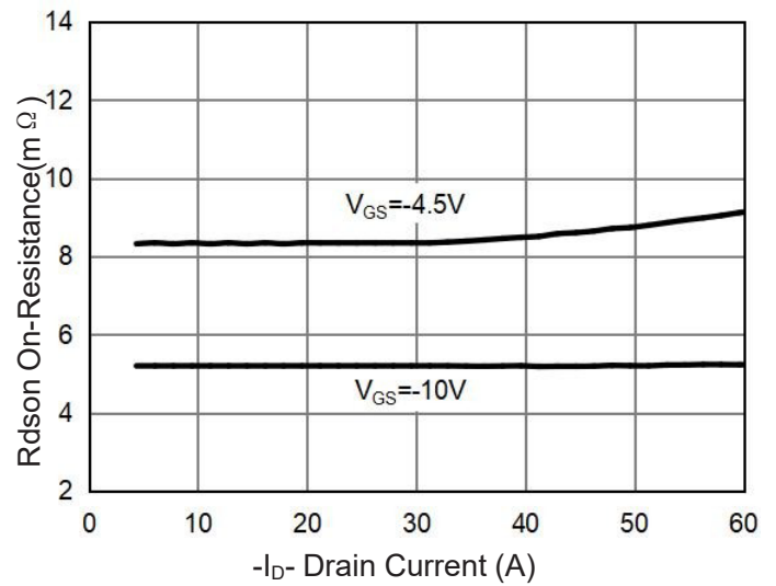
Figure 4 Drain-Source On-Resistance
