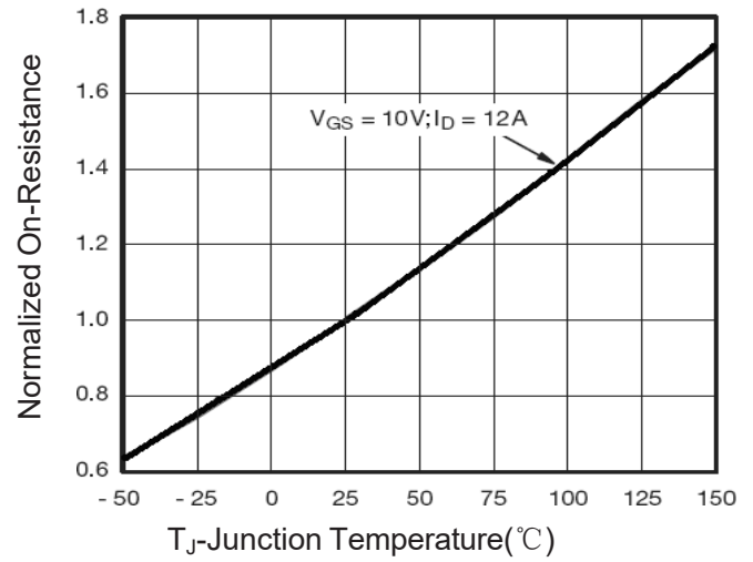
Figure 4 Rdson-Junction Temperature
