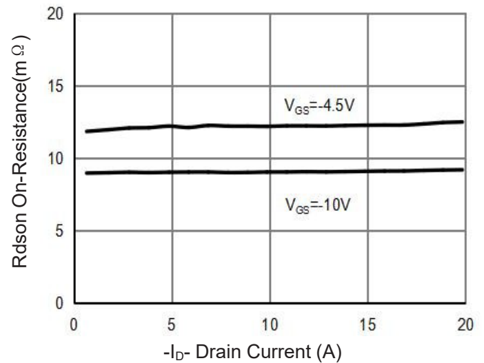
Figure 6 Drain-Source On-Resistance
