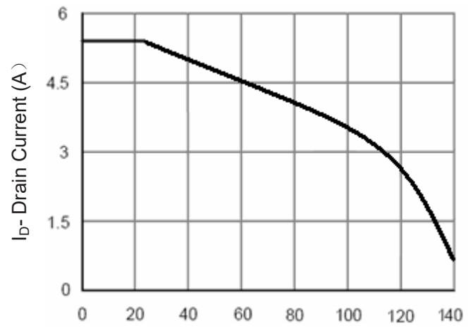
Figure 4 Drain Current
