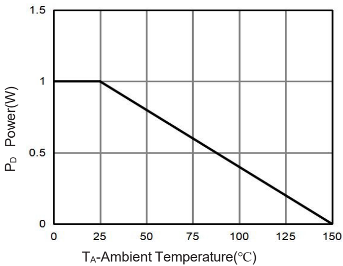
Figure 3 Power Dissipation
