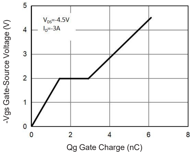
Figure 9 Gate Charge
