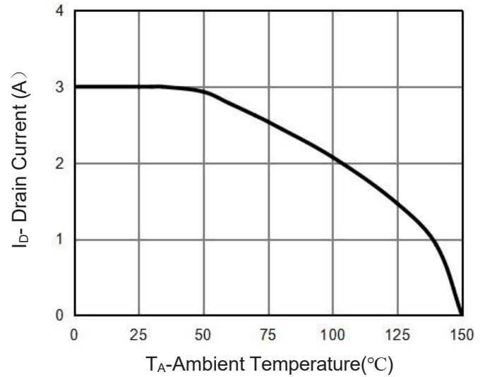
Figure 4 Drain Current
