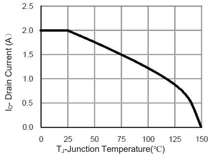
Figure 4 Drain Current
