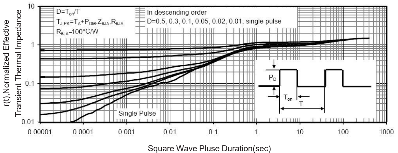
Figure 16 Normalized Maximum Transient Thermal Impedance
