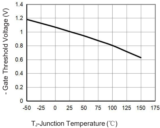
Figure 15 V GS(th) -Junction Temperature
