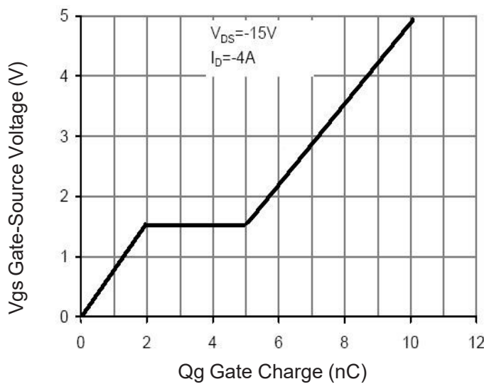
Figure 11 Gate Charge
