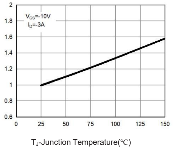
Figure 8 Drain-Source On-Resistance
