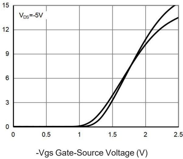
Figure 7 Transfer Characteristics
