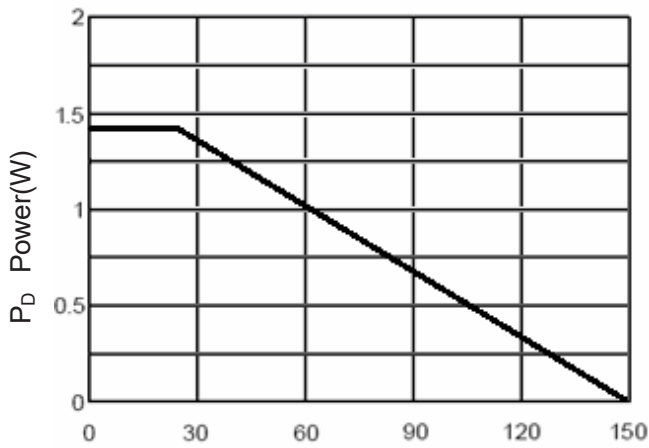
Figure 3 Power Dissipation
