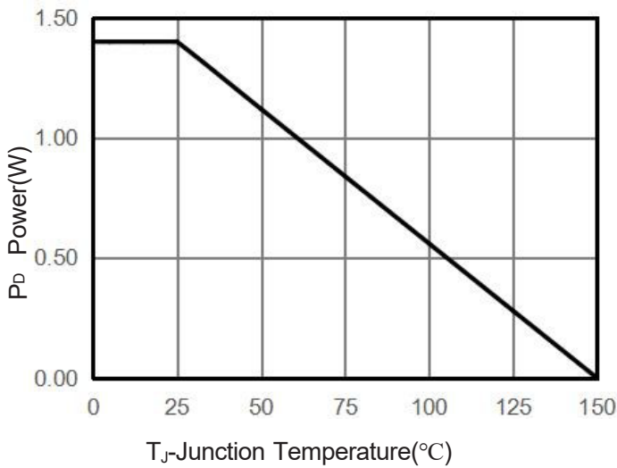
Figure 3 Power Dissipation
