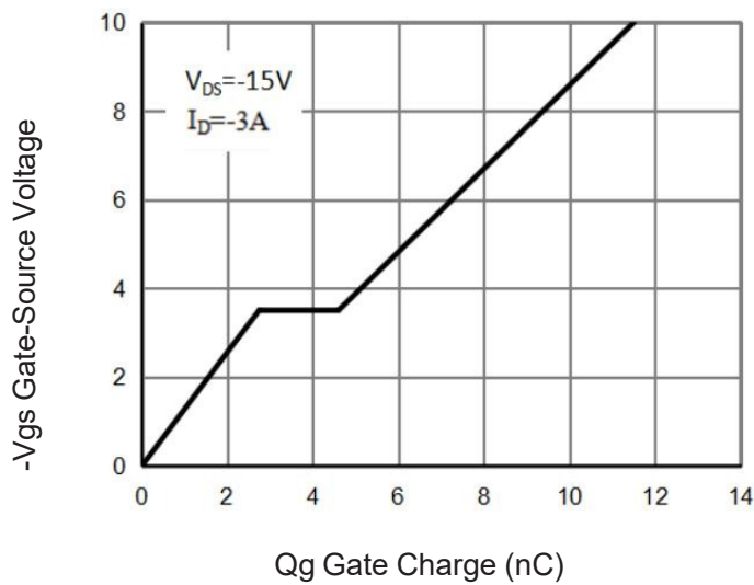
Figure 11 Gate Charge
