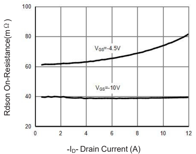
Figure 6 Drain-Source On-Resistance
