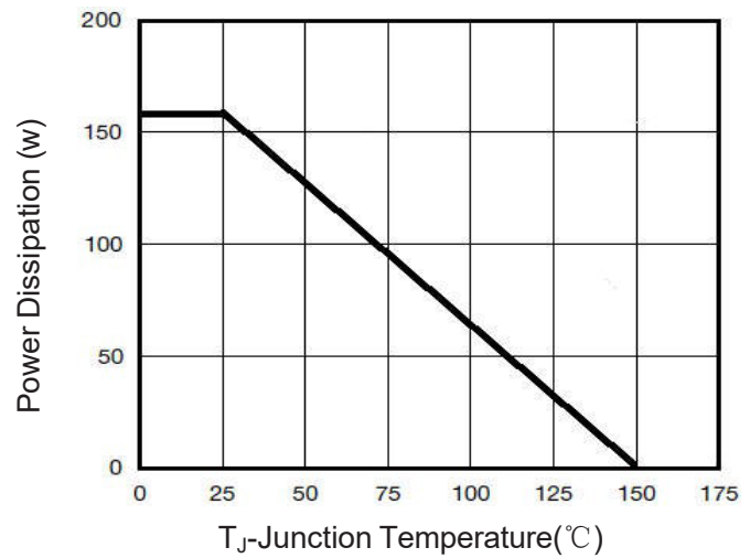
Figure 10 Power De-rating
