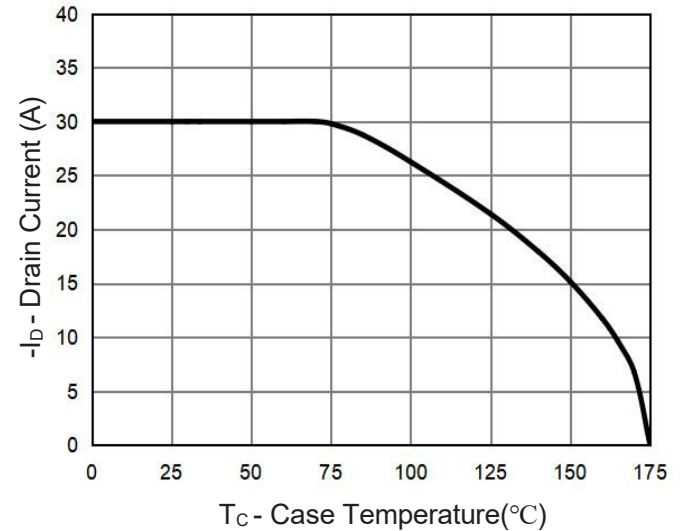
Figure 10 Drain Current De-rating
