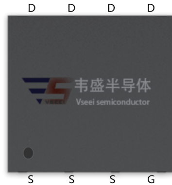
DFN3x3
