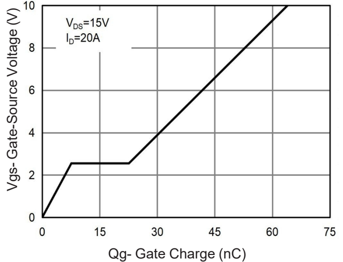
Figure 5 Gate Charge
