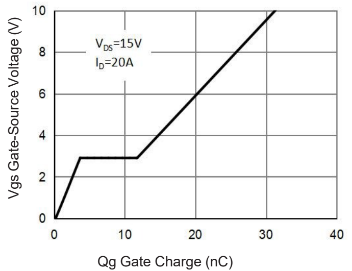
Figure 5 Gate Charge
