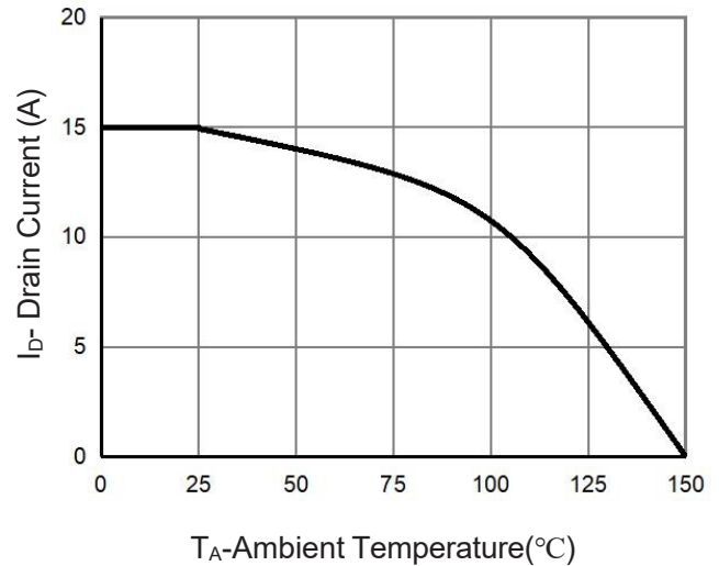
Figure10 ID Current- Ambient Temperature
