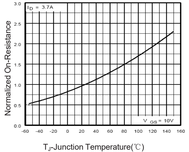
Figure 4 Rdson-Junction Temperature
