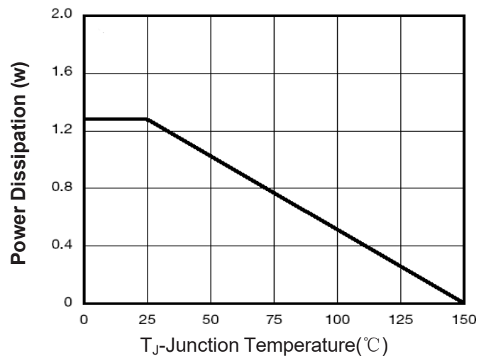
Figure 10 Power De-ratin
