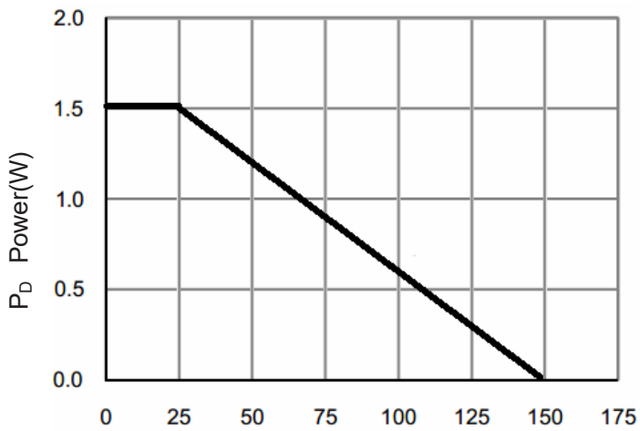
Figure 3 Power Dissipation
