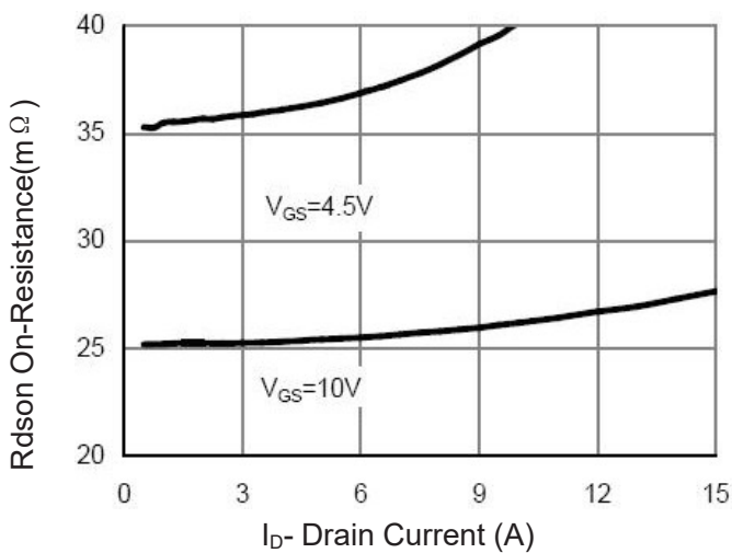
Figure 5 Drain-Source On-Resistance
