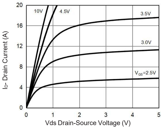
Figure 5 Output Characteristics
