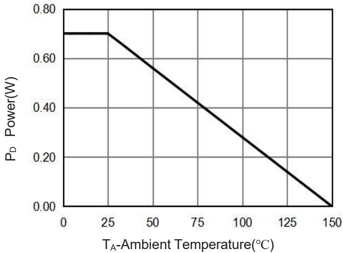
Figure 3 Power Dissipation
