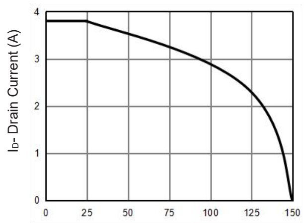
T C -Case Temperature(°C) Figure 10 Current De-rating
