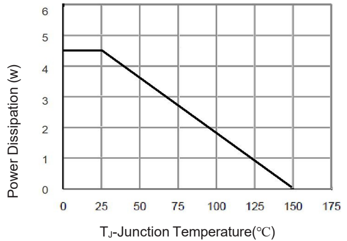
Figure 10 Power De-rating
