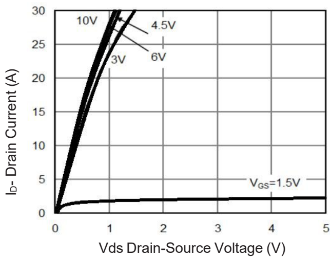
Figure 5 Output Characteristics
