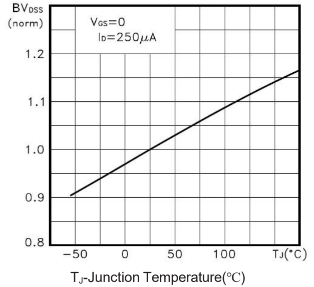
Figure 9 BV DSS vs Junction Temperature
