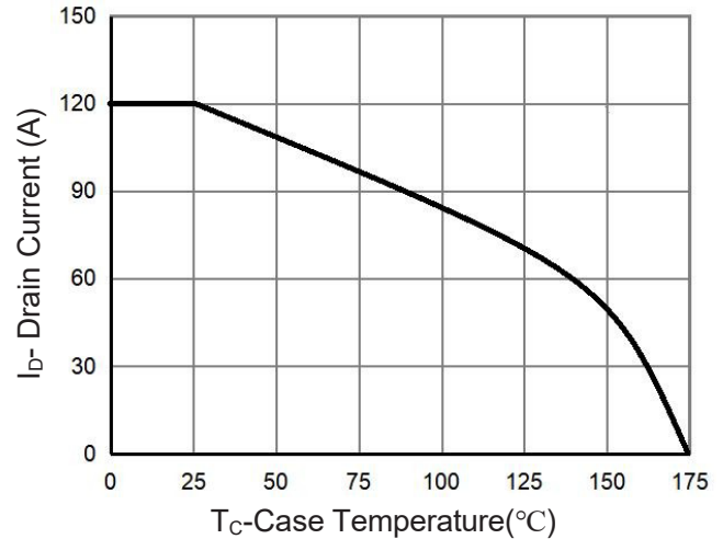
Figure 9 Current De-rating
