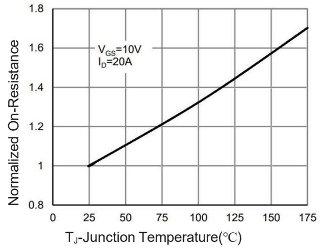
Figure 4 Rdson-Junction Temperature
