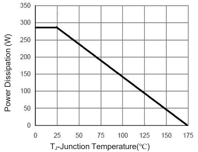
Figure 9 Power De-rating
