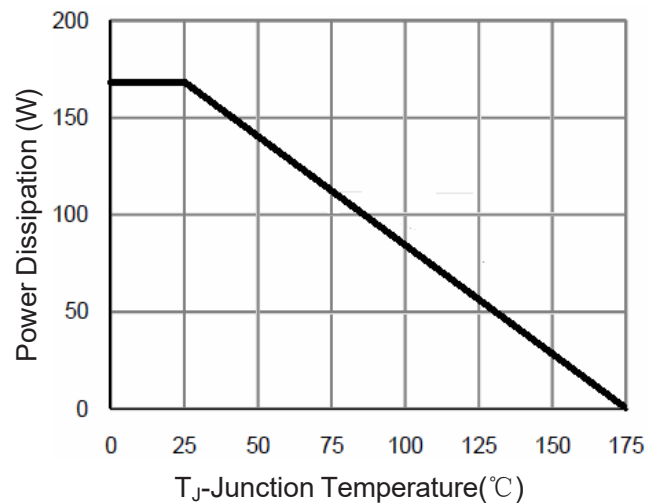
Figure 10 Power De-rating
