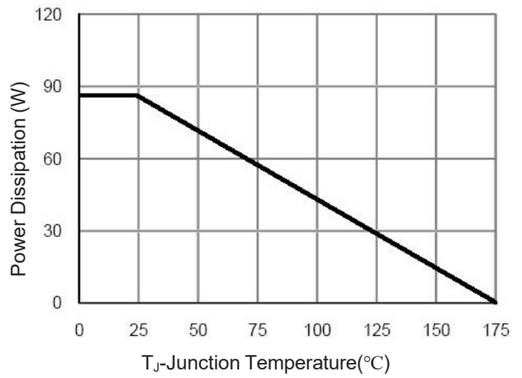
Figure 9 Power De-rating
