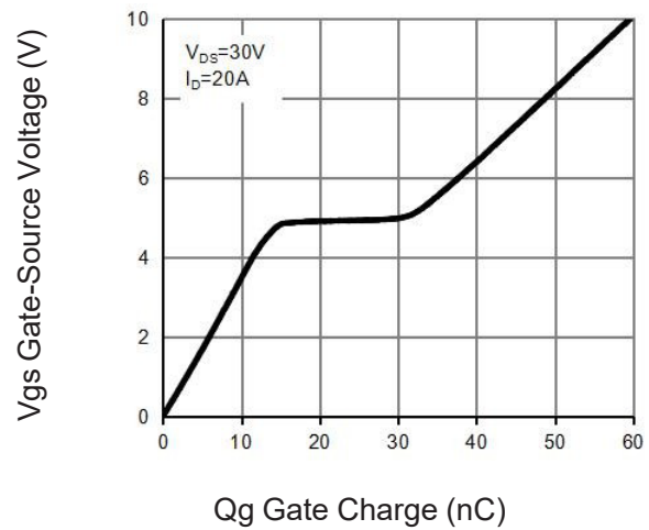
Figure 5 Gate Charge
