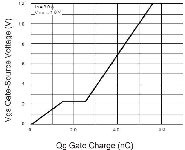
Figure 5 Gate Charge
