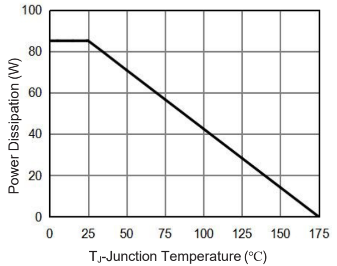
Figure 9 Power De-rating
