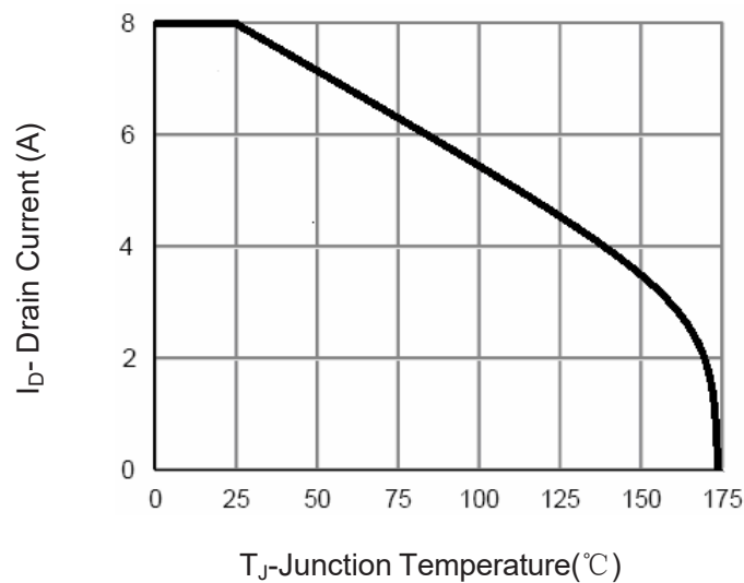
Figure 11 Current De-rating
