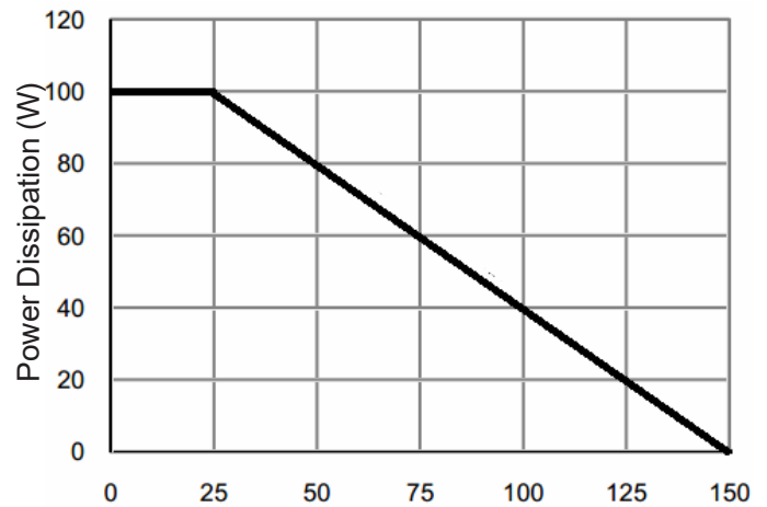
Figure 9 Power De-rating
