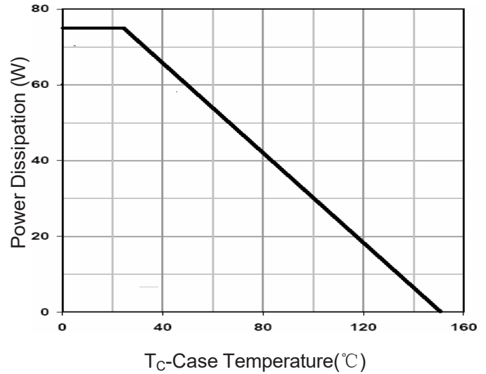
Figure 9 Power De-rating
