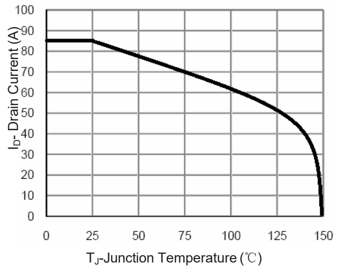
Figure 10 Current De-rating
