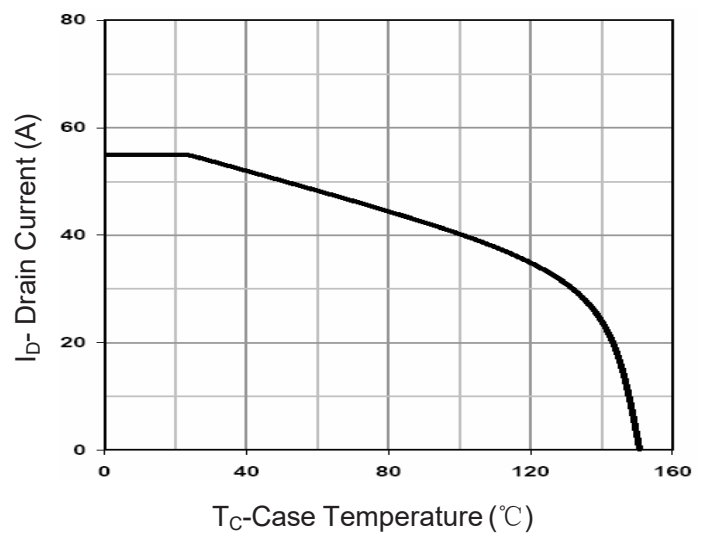
Figure 10 Current De-rating
