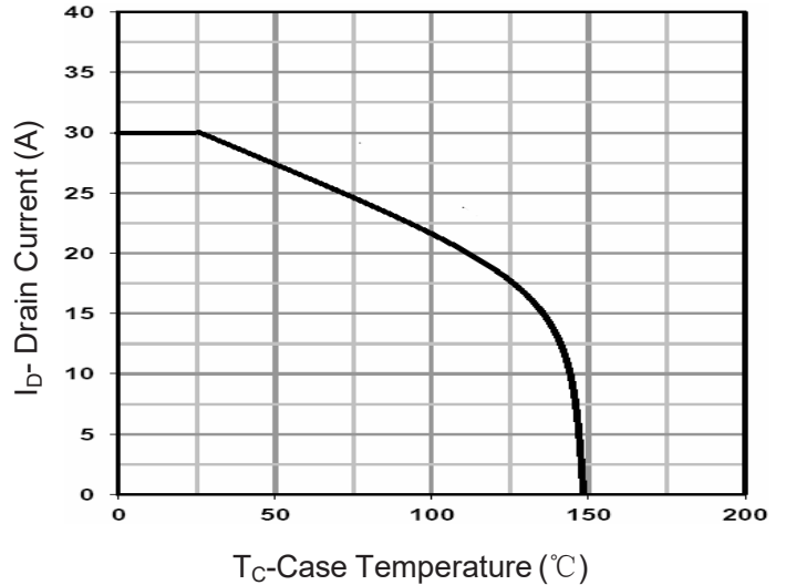
Figure 10 Current De-rating
