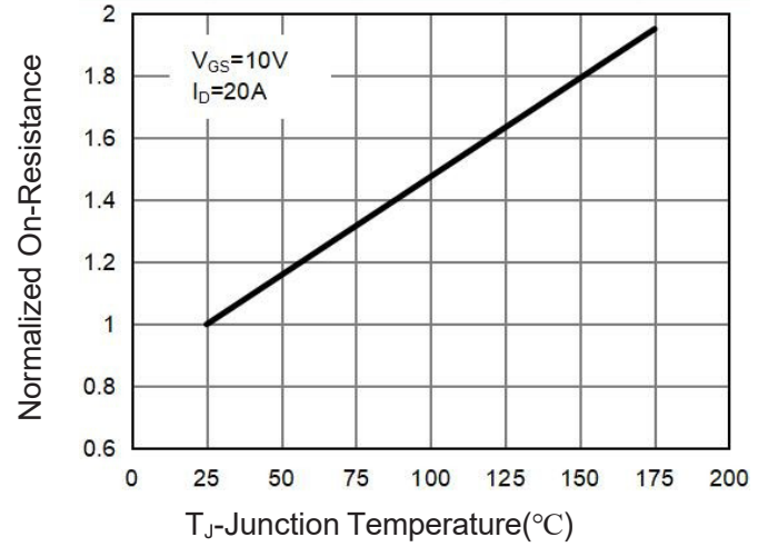
Figure 4 Rdson-Junction Temperature
