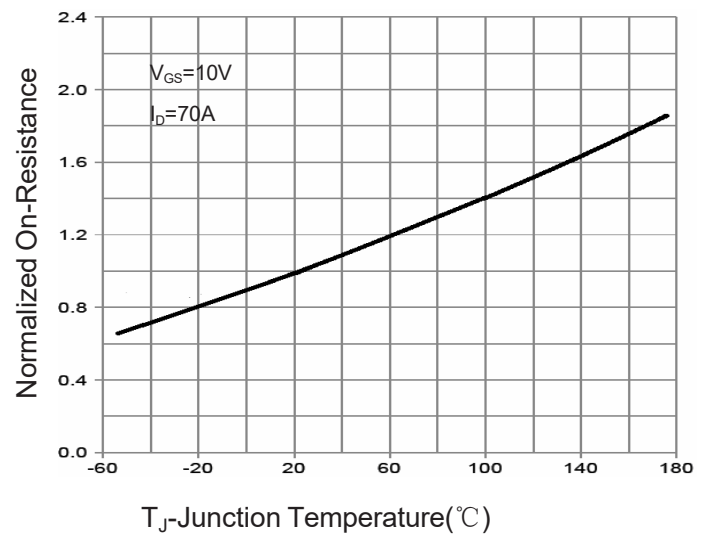
Figure 4 Rdson-Junction Temperature
