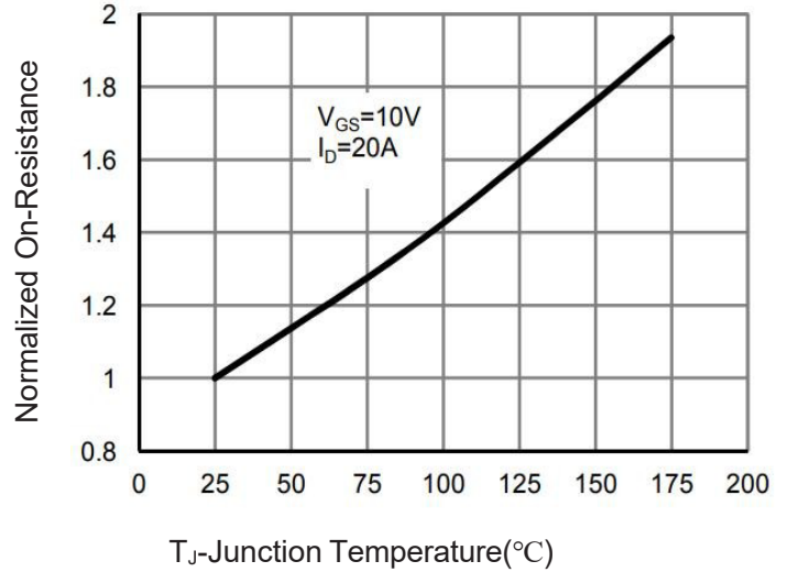
Figure 4 Rdson-Junction Temperature
