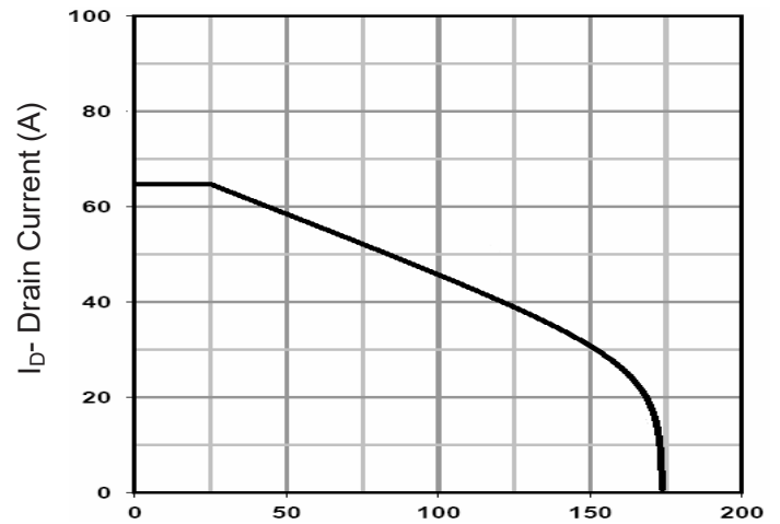
Figure 9 Current De-rating
