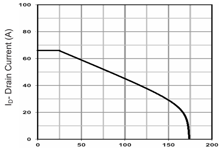
Figure 9 Current De-rating
