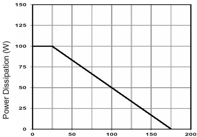
Figure 7 Power De-rating
