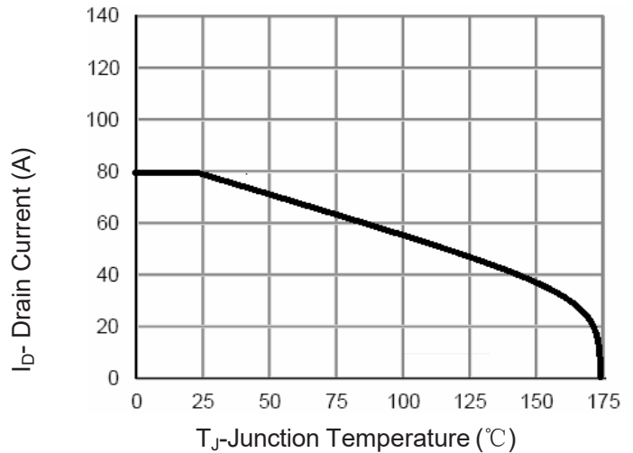
Figure 10 Current De-rating
