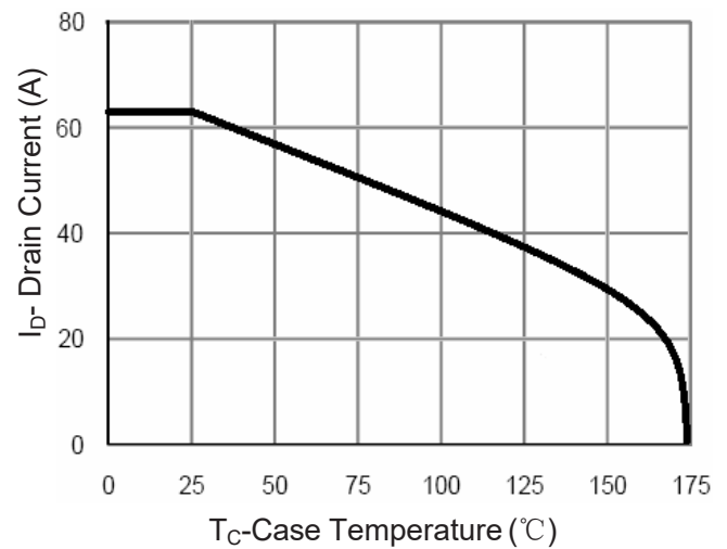
Figure 10 Current De-rating
