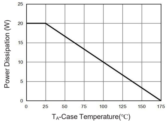
Figure 9 Power De-rating
