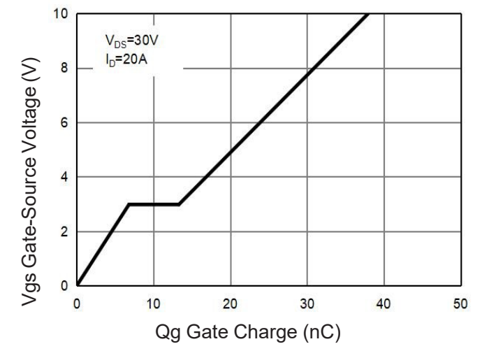
Figure 5 Gate Charge
