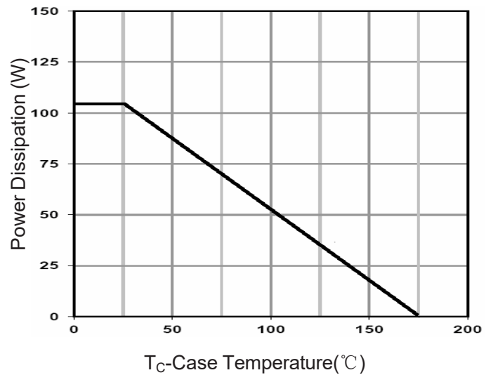
Figure 9 Power De-rating
