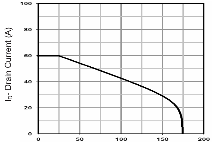
T_C -Case Temperature (°C) Figure 9 Current De-rating
